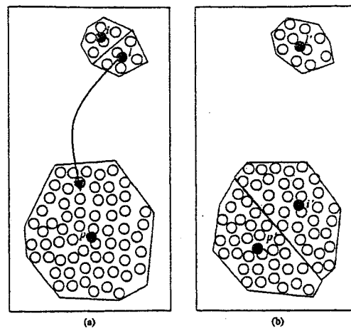
Fig. 1. (a) A situation where the codewords are badly distributed. The arrow indicates a possible solution. (b) A better distribution.
