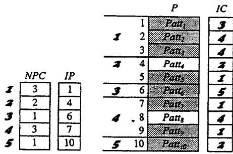
Fig. 11. Initial situation. Only the arrays and the matrices involved in the sorting operation are reported.
