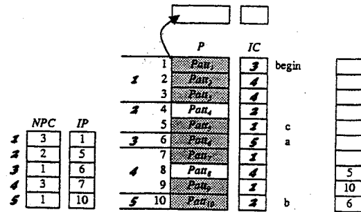
Fig. 12. Sorting: stack creation.
