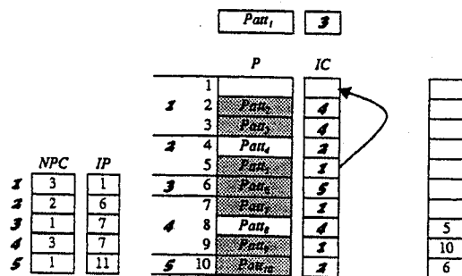
Fig. 13. Emptying of the stack (I).
